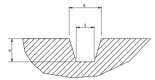
Lateral Grooves
