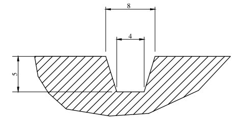
Lateral & Circumferential Grooves
