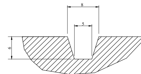
Lateral Grooves
