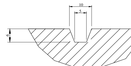
Circumferential Grooves
