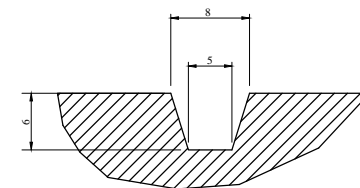
Lateral Grooves
