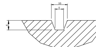
Circumferential Grooves
