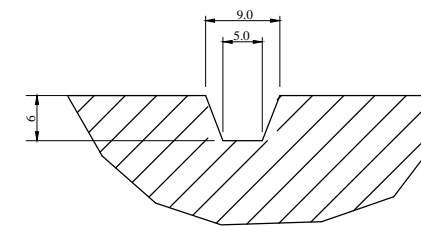
Circumferential Grooves
