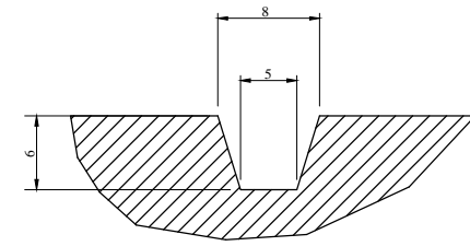
Lateral Grooves
