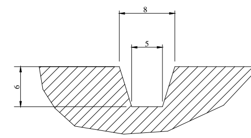
Lateral Grooves
