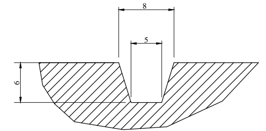
Lateral Grooves
