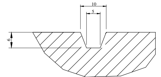
Circumferential Grooves
