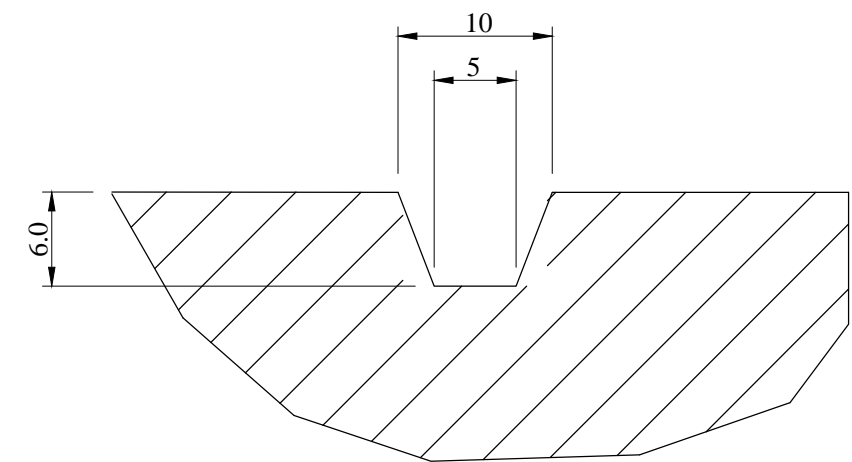
Circumferential Grooves
