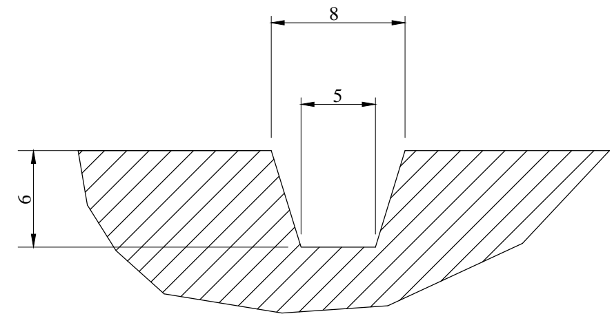
Lateral Grooves
