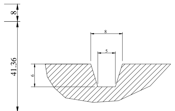
Lateral Grooves
