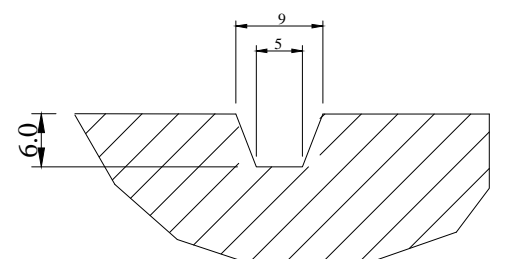
Circumferential Grooves
