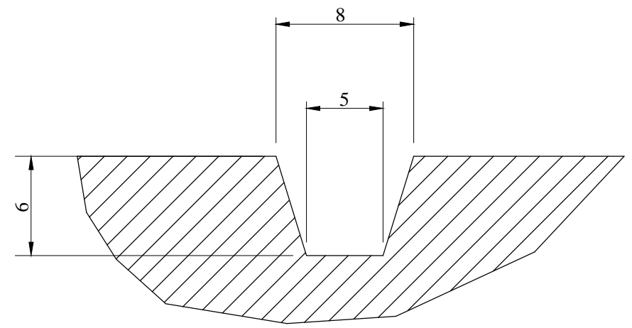
Lateral Grooves
